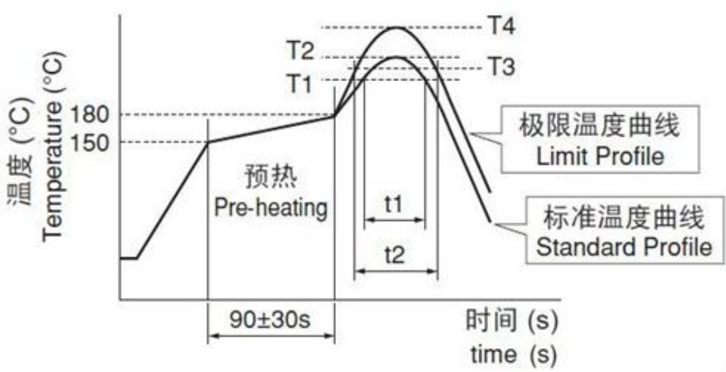
回流焊温度曲线 Reflow Soldering Temperature Profile
